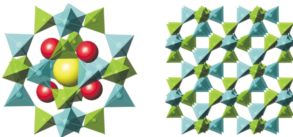
Fig. 2 The sodalite structure, Na 8 [AlSiO 4 ] 6 Cl 2 . The linking of alternate SiO 4 (green) and AlO 4 (blue) tetrahedra forms a body centred arrangement of framework β cages, right. Each cage contains a central anion (yellow) surrounded tetrahedrally by cations (red), left; the cations also interact strongly with three framework oxygen atoms to produce a distorted tetrahedral environment for these ions.
