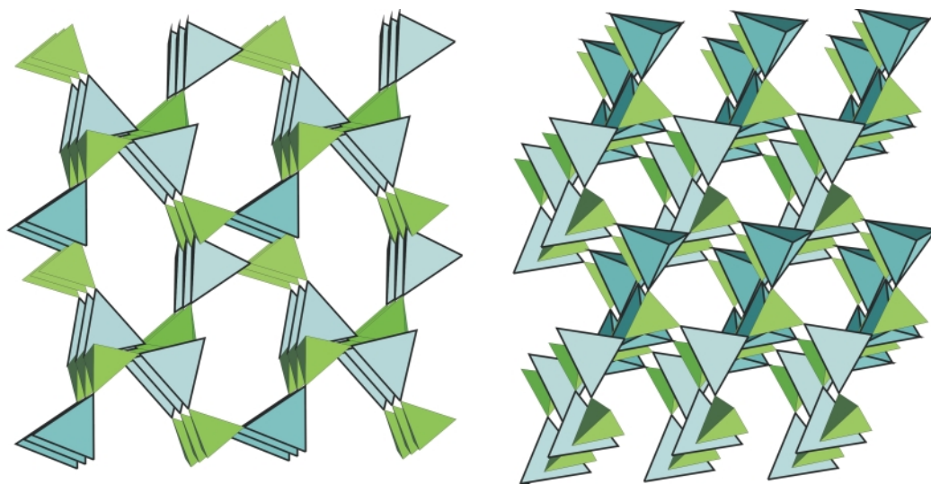
Fig. 9 The zeolite ABW framework constructed using alternating silicate (cyan) and aluminate (green) tetrahedra viewed along the c (left) and b (right) directions.
