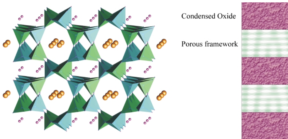
Fig. 11 The JBW framework of \text{Na}_2\text{Rb}[\text{Al}_3\text{Ge}_3\text{O}_{12}] (left) viewed down the c direction showing the main 8-ring channels. The framework consists of alternating \text{AlO}_4 tetrahedra (cyan) and \text{GeO}_4 tetrahedra (green); sodium atoms are purple and rubidium gold. The schematic on the right represents the alternating layers of non-hydrated oxide (purple) and porous channels (green).
