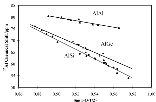
Fig. 5 Typical structure–MAS NMR chemical shift relationship derived from sodalite structures with variations in the ^{27}\text{Al} chemical shift position plotted as a function of \sin[(\text{Al–O–T})/2] . (T = Al, Ge or Si). This sine function has widely been used in the literature to describe effect of the T–T separation on chemical shift.
