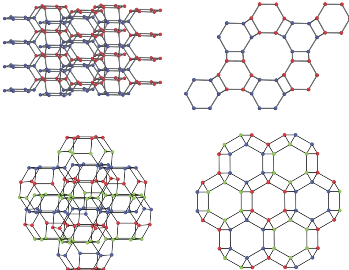
Fig. 7 The stacking sequence of 6-rings in the sodalite (ABCABC ...), bottom, and the cancrinite (ABABAB ...), top, structures and the derived pore structures (right). Tetrahedral atoms in the two structures are coloured red, green and blue to represent the different positions of the vertically stacked layers.
