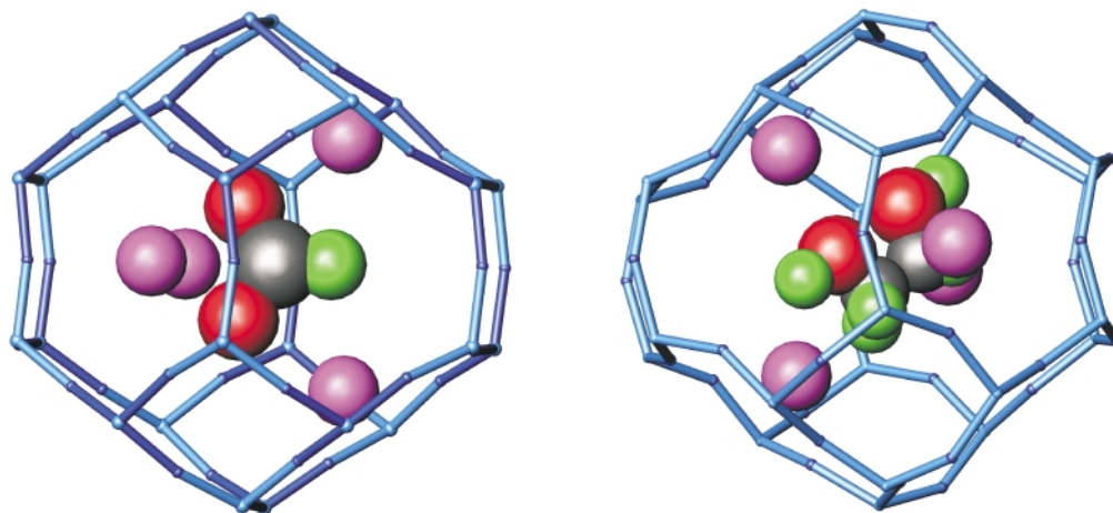
Fig. 4 The sodalite cage of formate aluminogermanate sodalite \text{Na}_8[\text{AlGeO}_4]_6(\text{HCO}_2)_2 showing the position of the formate ion as determined from powder neutron diffraction (left); the sodium ions are also shown (magenta). The sodalite cage of ethylene glycol silica sodalite showing the position of the organic species is given at the right; the sodium ions are also shown (magenta). Key: carbon, grey; oxygen, red and hydrogen, green.
