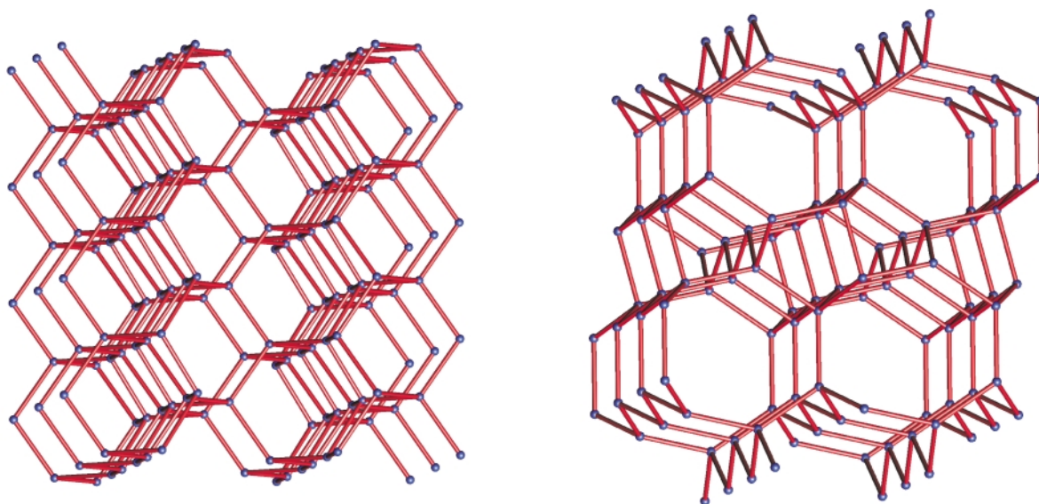
Fig. 13 The frameworks of the CAS (left) and BIK (right) zeolite structures. The framework oxygen atoms are not shown and the tetrahedral sites are linked directly.
