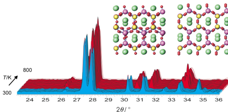
Fig. 10 Phase transition in the CsCoPO 4 ABW structure. Variable temperature powder X-ray diffraction data show a marked change in the pattern at 170 °C distinguished by the blue/red shading. The two structures viewed down the main channel are shown. Left: the low temperature form, space group P2 1 /a , with a twisting of the TO 4 units in opposite directions with respect to each in successive layers. Right: the high temperature form, space group Pn2 1 a .
