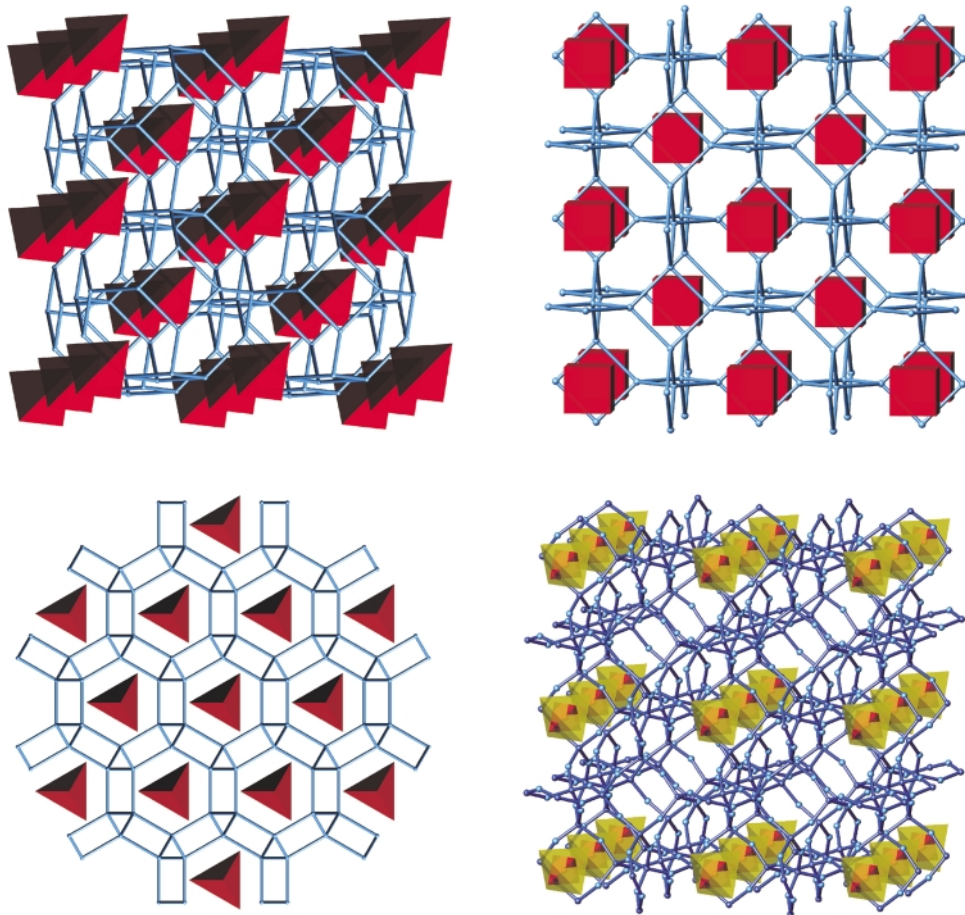
Fig. 3 Arrays of inorganic blocks in sodalite derived structures. Anti-clockwise from top left: face centred array of M_4X tetrahedral units as in M_8[BeSiO_4]_6X_2 viewed close to [100] , face centred cubic array of M_4X tetrahedral units as in M_8[BeSiO_4]_6X_2 viewed down [111] , body centred array of interpenetrating double M_4(AO_4) tetrahedral units as in noselites M_8[AlSiO_4]_6AO_4 and face centred array of M_4X_4 cubes as in bicchulite M_8[AlO_2]_{12}X_8 .
