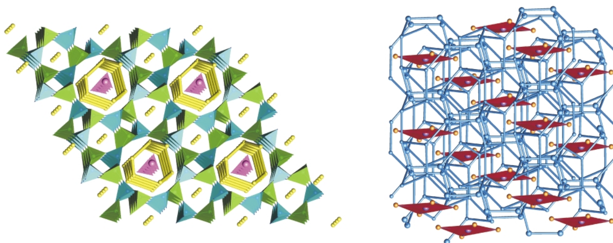
Fig. 15 Representations of the scapolite structure (right) showing the distribution of square planar M_4X units in three dimensions and cancrinite (left) showing triangular anions in the channels surrounded by the cations.
