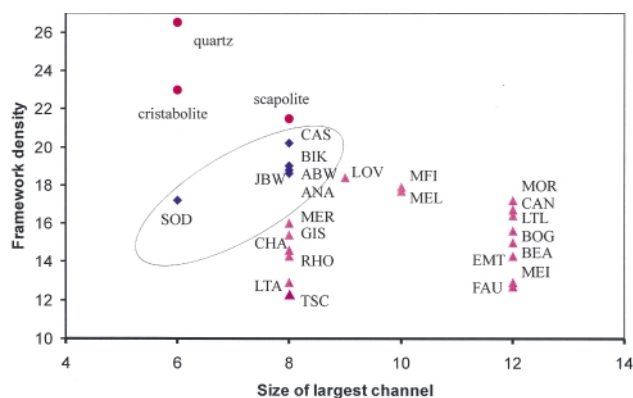
Fig. 1 Framework density versus maximum ring opening size for a range of tetrahedral frameworks. Frameworks are divided into three regions corresponding to dense oxide-like structures (●), open porous zeolites (▲) and intermediate structure types (◆).
