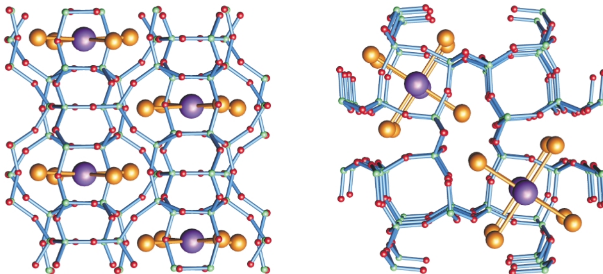
Fig. 14 The scapolite structure, M_4[T_4O_8]X , viewed down the c (left) and the b direction (right). The framework bonds are shown in blue, the anion (X) as the purple sphere and the cation (M) as gold spheres.
