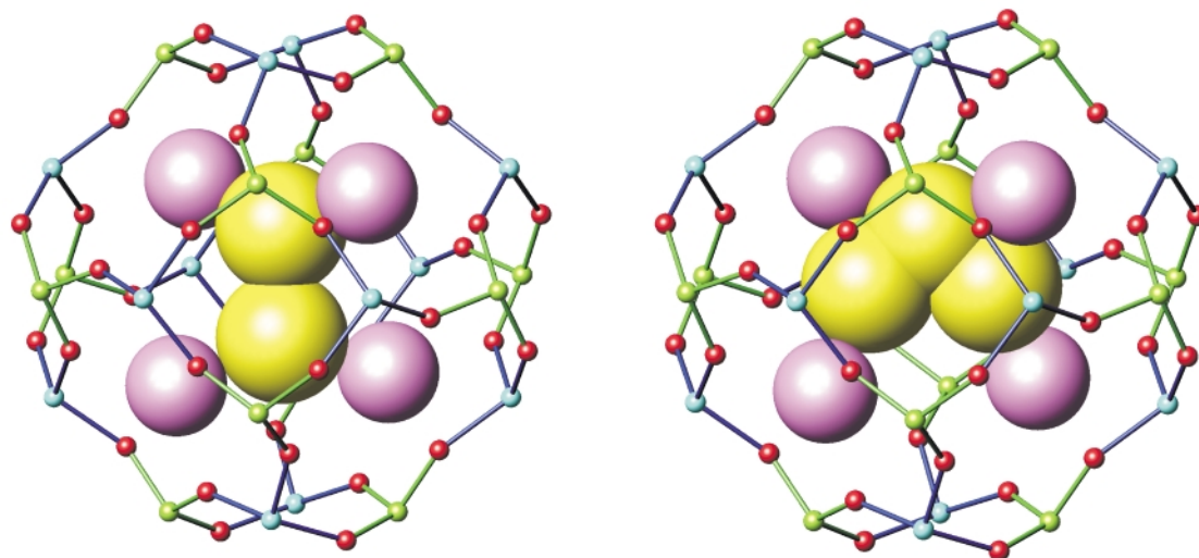
Fig. 6 The structures of the ultramarines yellow Na_{6.7}[AlSiO_4]_6(S_2)_{0.67} and blue Na[AlSiO_4]_6(S_3) derived from the analysis of S-edge EXAFS and powder neutron/X-ray diffraction data. Sulfur atoms are yellow, sodium ions magenta.
