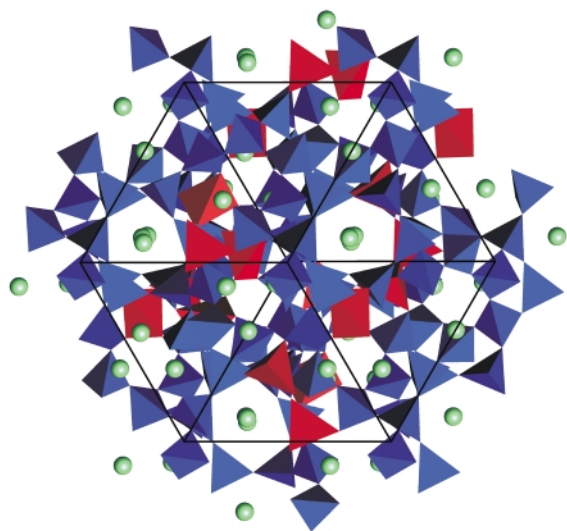
Fig. 12 The analcime (ANA) structure of \text{Cs}_2\text{MSi}_5\text{O}_{12} , \text{M} = \text{Co} or \text{Ni} , viewed down the main pore direction. The \text{SiO}_4 tetrahedra are shown in blue and \text{MO}_4 in red; caesium ions are green.
